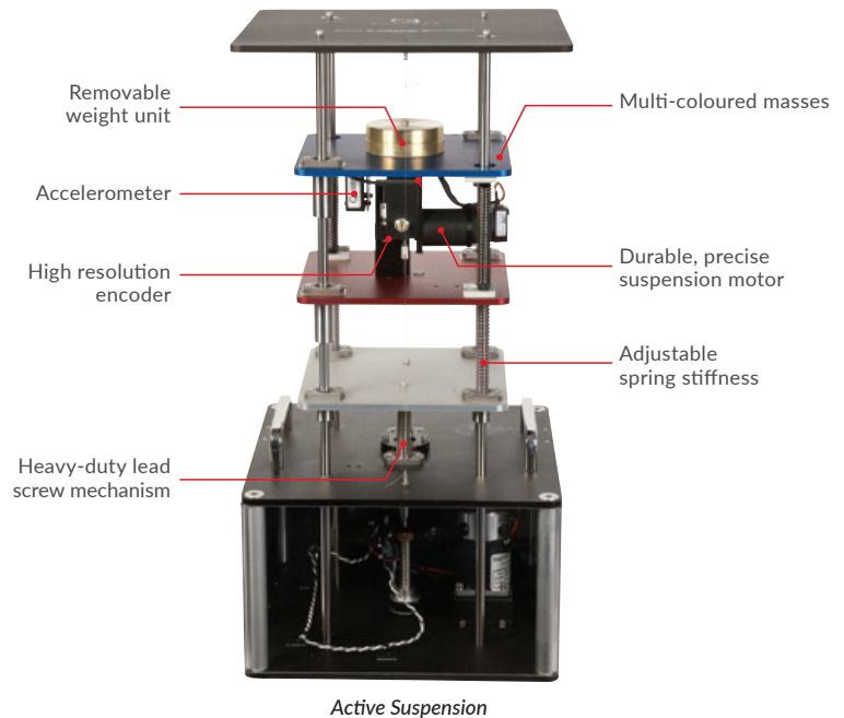
Active Suspension
