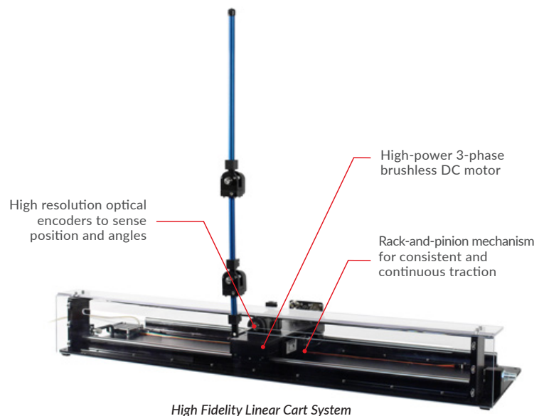
High Fidelity Linear Cart System
